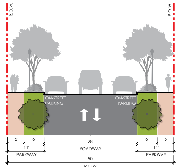
RESIDENTIAL STREET CROSS SECTION (NTS)
